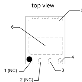
Package Outline
